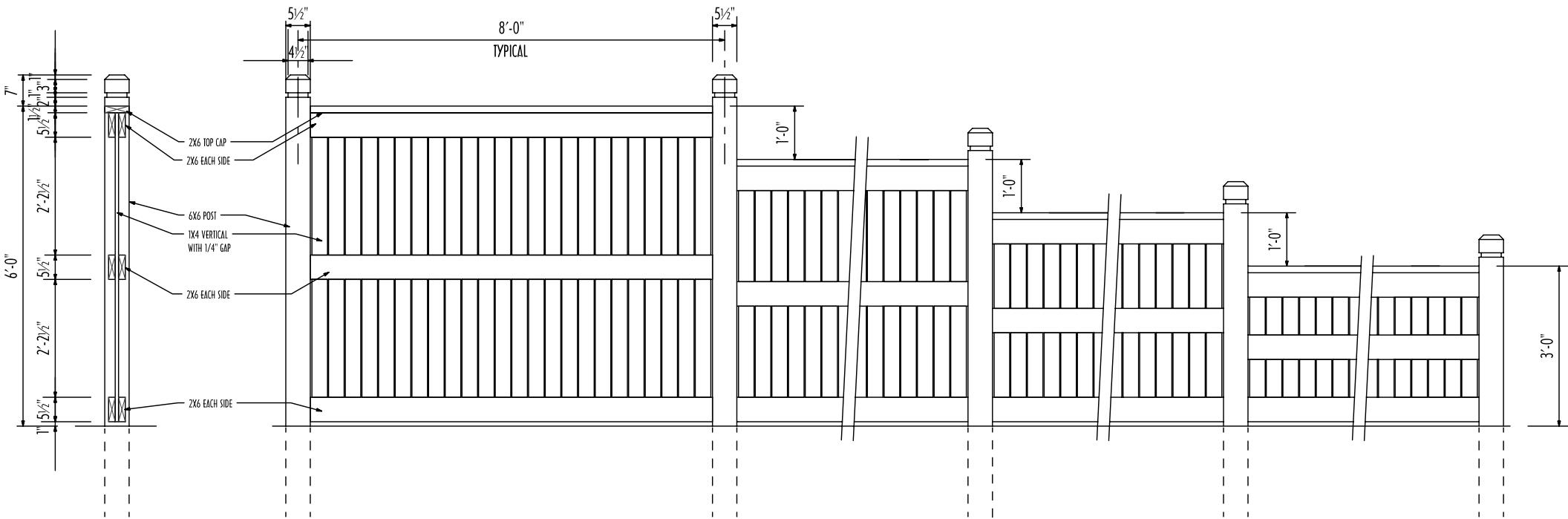
SECTION VIEW
