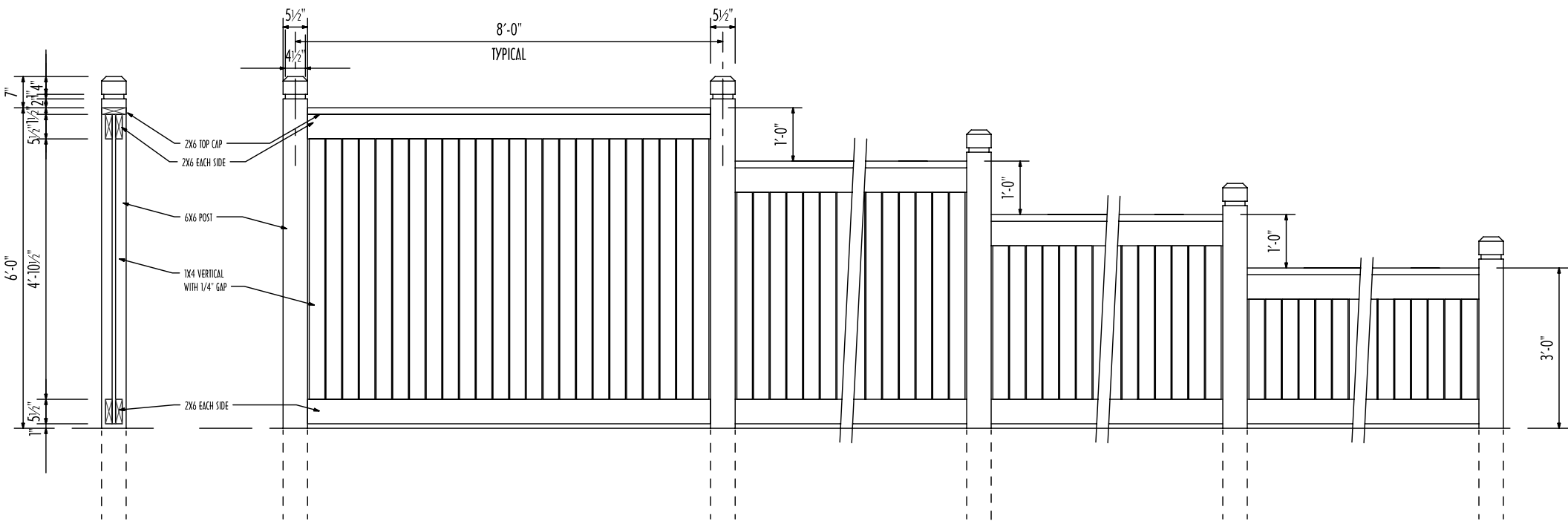
SECTION VIEW
